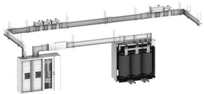
Fig. E45 : A busway for high power distribution : Canalis KT (800 up to 1000 A)
