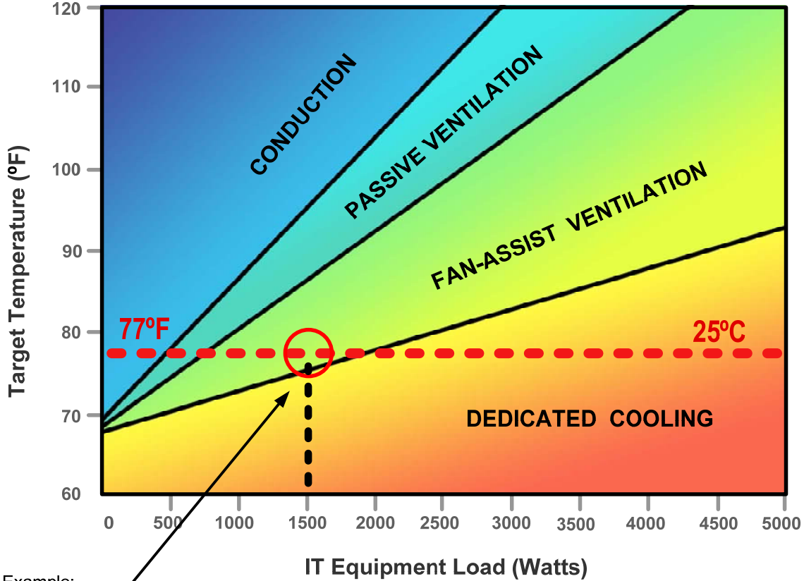
Figure 1 – Cooling method guide based on power load and target room temperature
