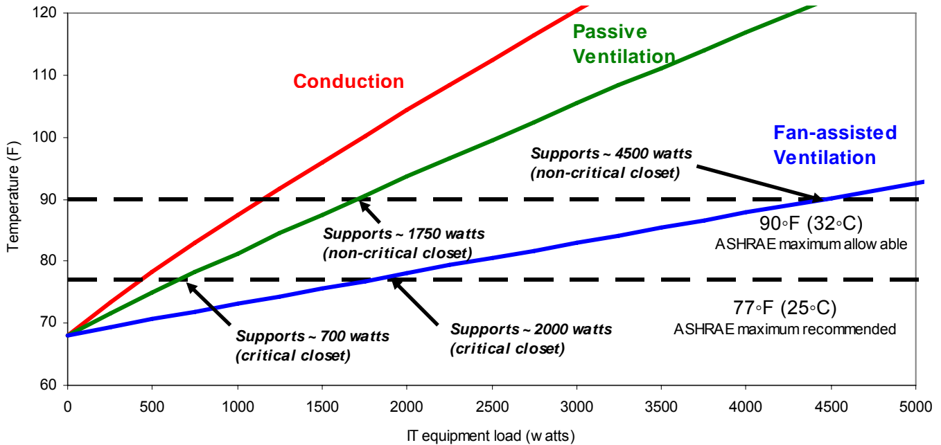
Figure 7 – Closet temperature versus IT load – passive and fan-assisted ventilation
