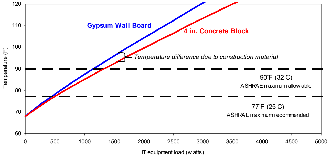
Figure 5 – Effect of construction material on conduction cooling performance
