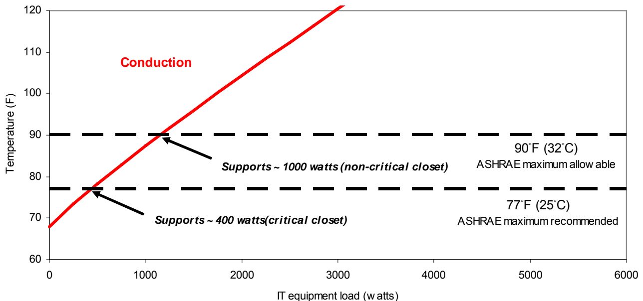
Figure 3 – Closet temperature versus IT equipment load: conduction performance
