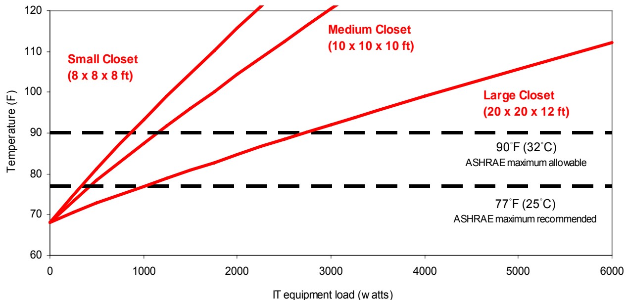
Figure 4 – Effect of closet dimensions on conduction cooling performance
