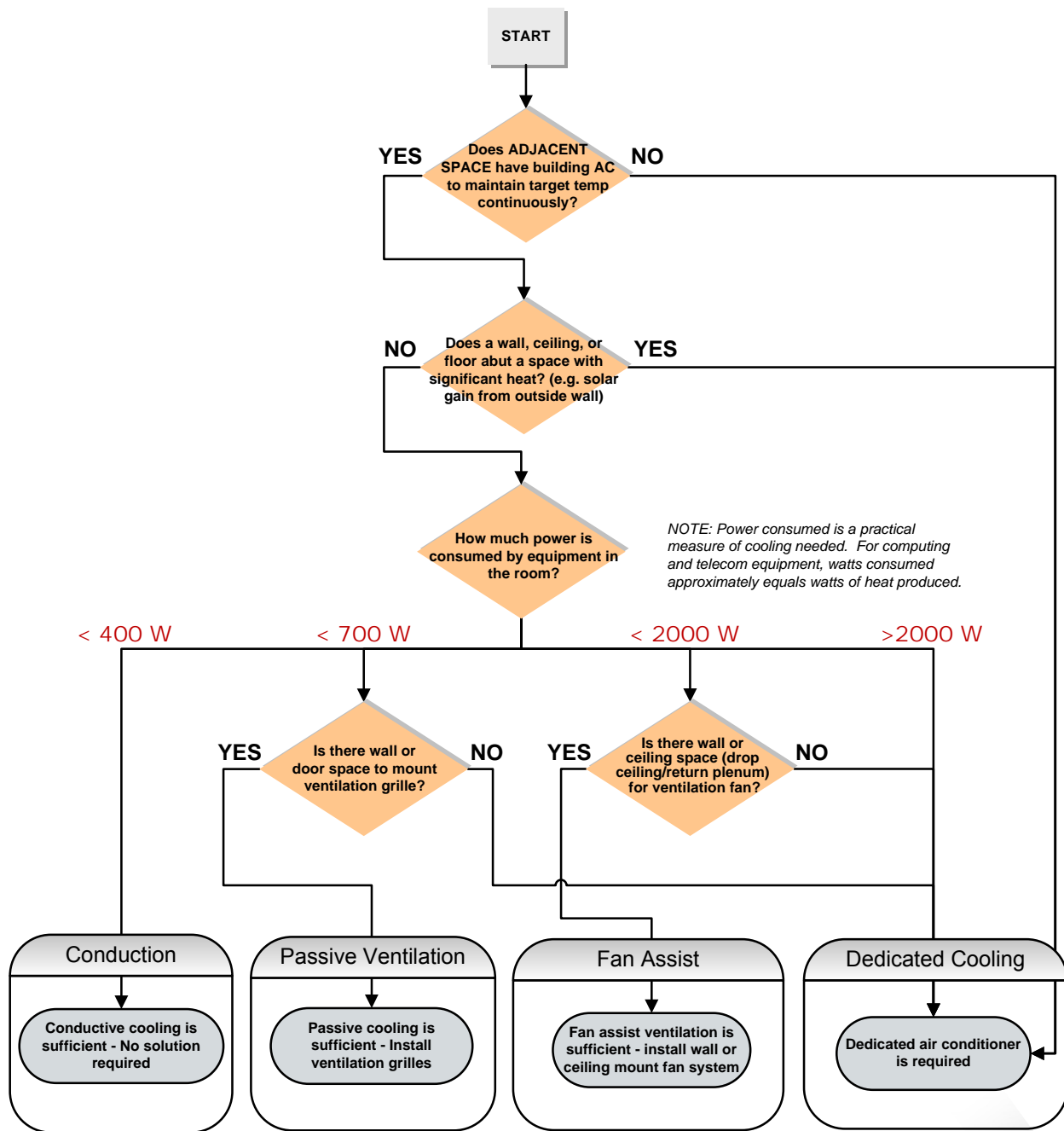
Figure 2 – Cooling method selection to maintain recommended ASHRAE temperature range of 68 - 77°F (20 - 25°C)
